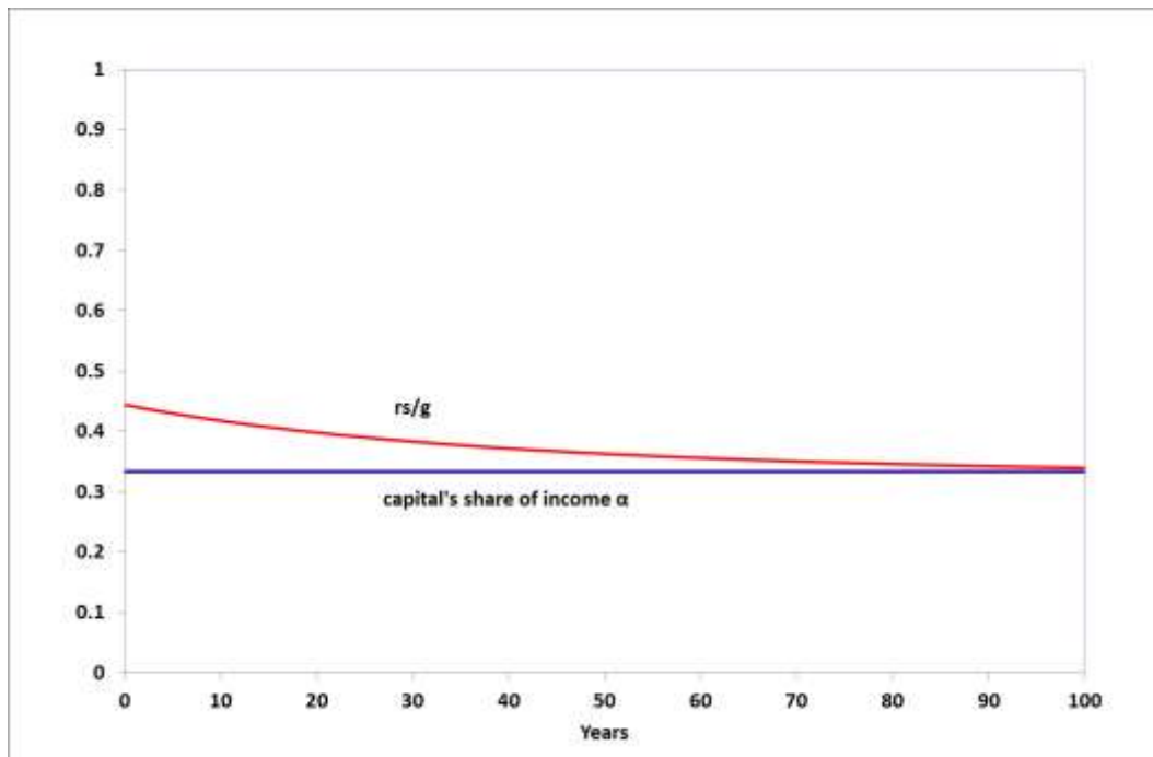
Figure 2b: Long-term convergence of capital's share of income with s and g held constant
